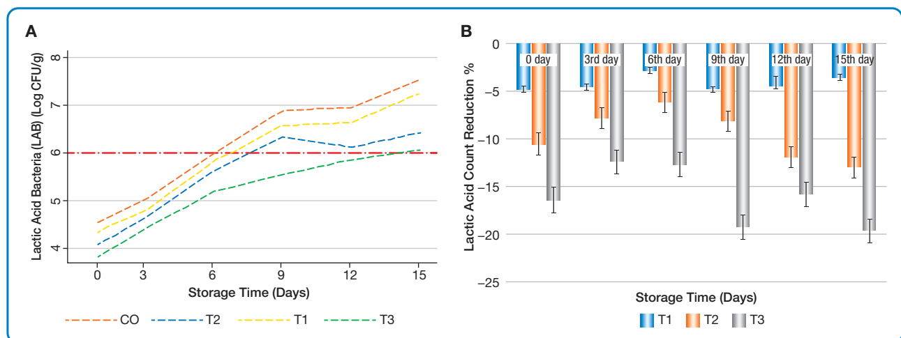
Figure 3. (A): Evolution of LAB (log 10 CFU/g) counts of control (CO) and pomegranate molasses-marinated chicken breast fillet groups; T1 (0.5% v/w), T2 (1% v/w) and T3 (1.5% v/w) stored at 4 °C, (B): Microbial reduction percentage of LAB
